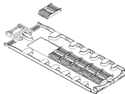
FOSC-D-TRAY-36/S96/L96/A96/RT24
