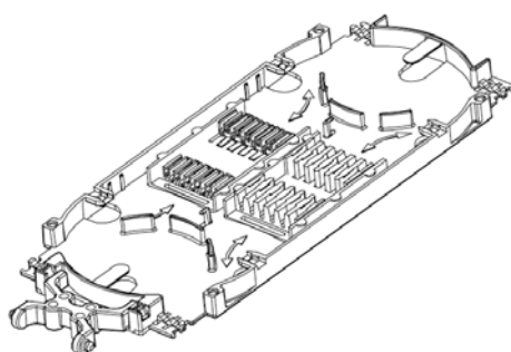
FOSC-A-TRAY-12/16/24
