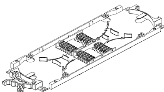
FOSC-B-TRAY-12/24
