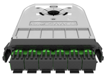
360G2 Singlemode Fiber Cassette 12 LC APC, no pigtails, iPatch Ready
